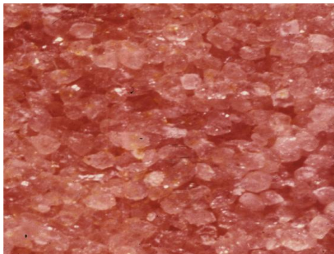
Fig. 1. Grains of the mineral quartz cemented together to form the rock sandstone.
