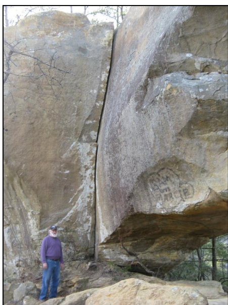
Fig. 7a. Large joint bounding the side of Sky Bridge.
